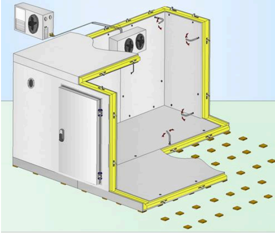
Panel layout of a modular cold room
